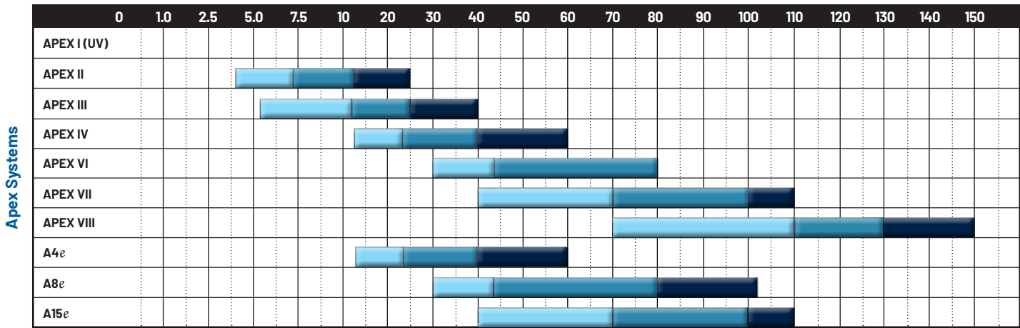
APEX & APEX e SYSTEM SIZING CHART
